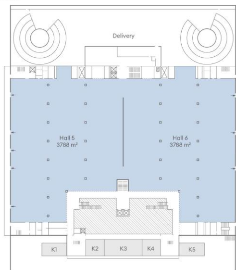
2nd Floor
